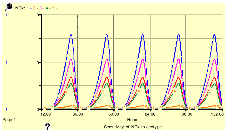
Figure 18: Sensitivity of NO x to habitat type in the simulation model. The numbers on each curve correspond to the habitat type being simulated within the model. (See Table 1 for key to habitat numbers).
