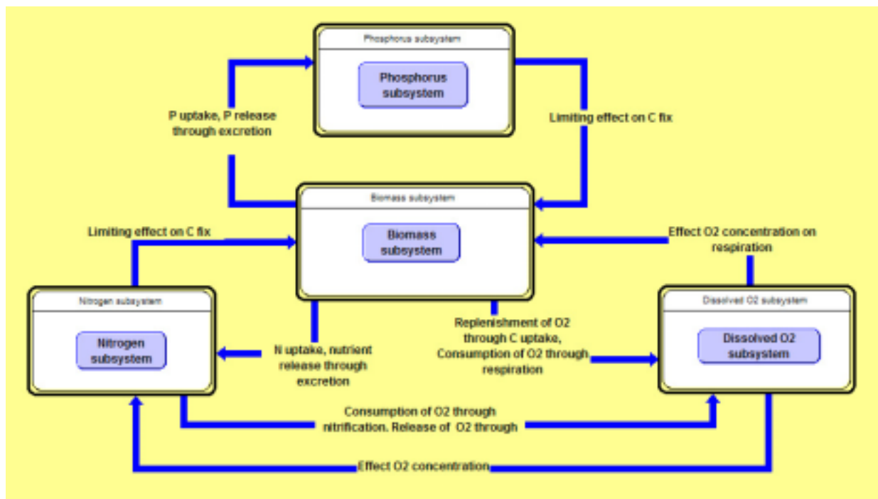
Figure 4: Summary diagram of the main components to the initial benthic habitat model. This structure is applied to each habitat using the field and literature data available to derive the interaction terms.
