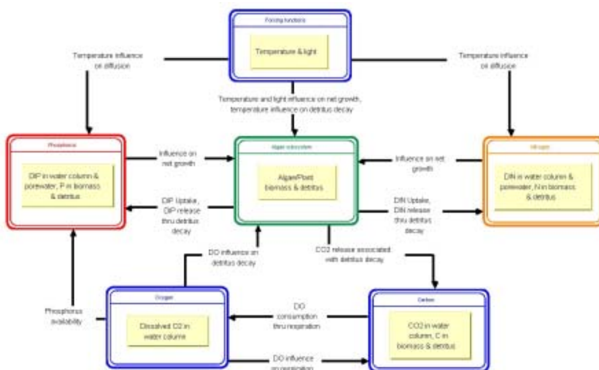
Figure 15: Component structure of second generation benthic model used for simulation of habitat nutrient responses relative to composition.
