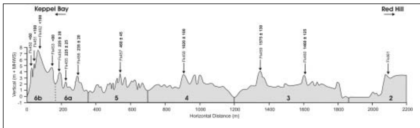
Figure 3: A surveyed cross-section of the beach ridge plain at Long Beach, on the western margin of Keppel Bay. Five accretion units (sets of ridges) are indicated by numbers (6b – 2).
