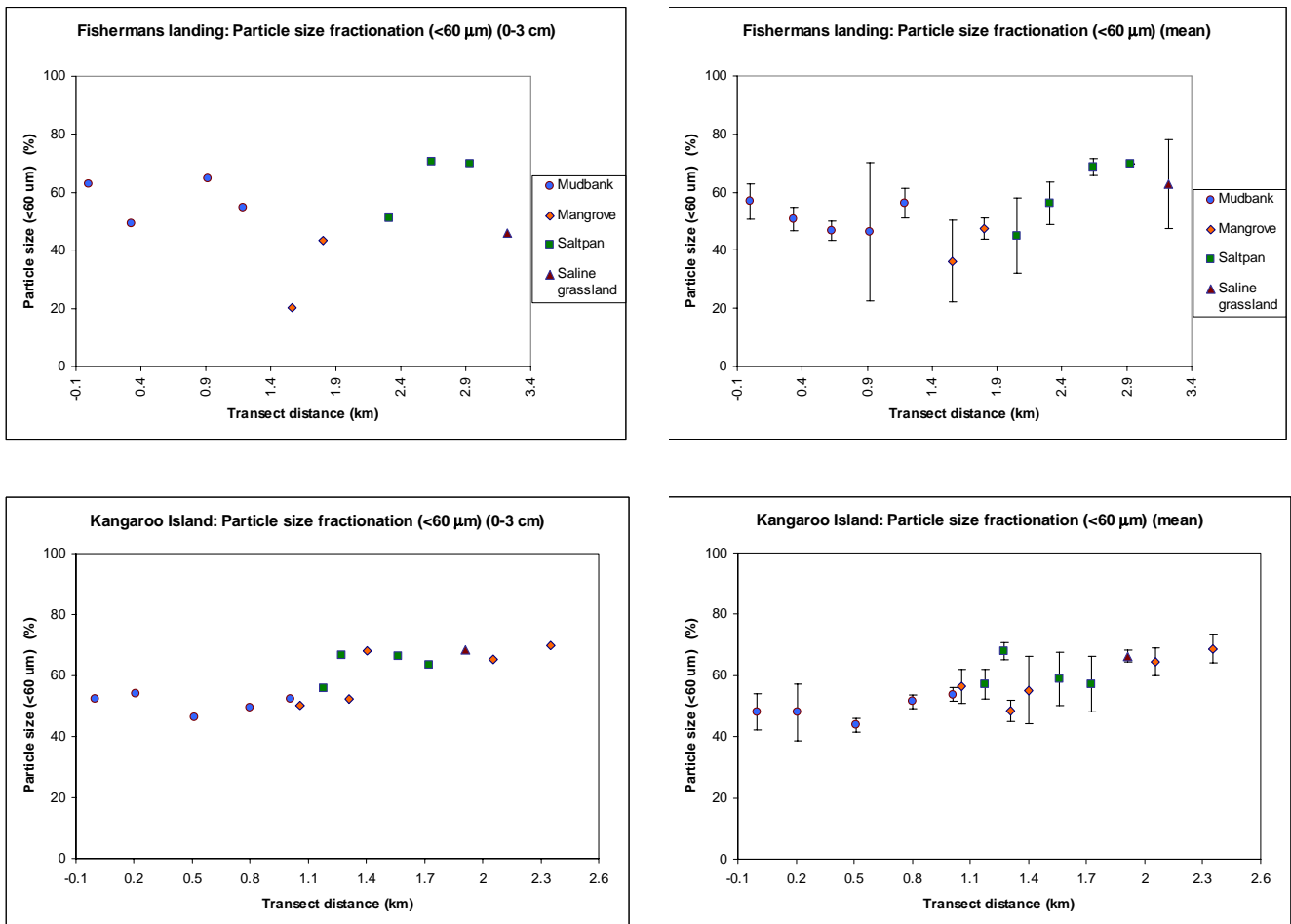
Figure 3.10. Transect particle size fractionation measurements <60 µm (surface 0–3 cm and mean depth profile) at Fisherman’s Landing and Kangaroo Island
