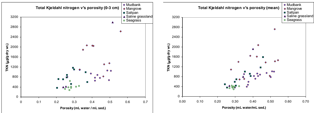
Figure 3.22. Relationships between total Kjeldahl nitrogen and porosity for surface (0–3 cm) and mean depth measurements from all sites combined
