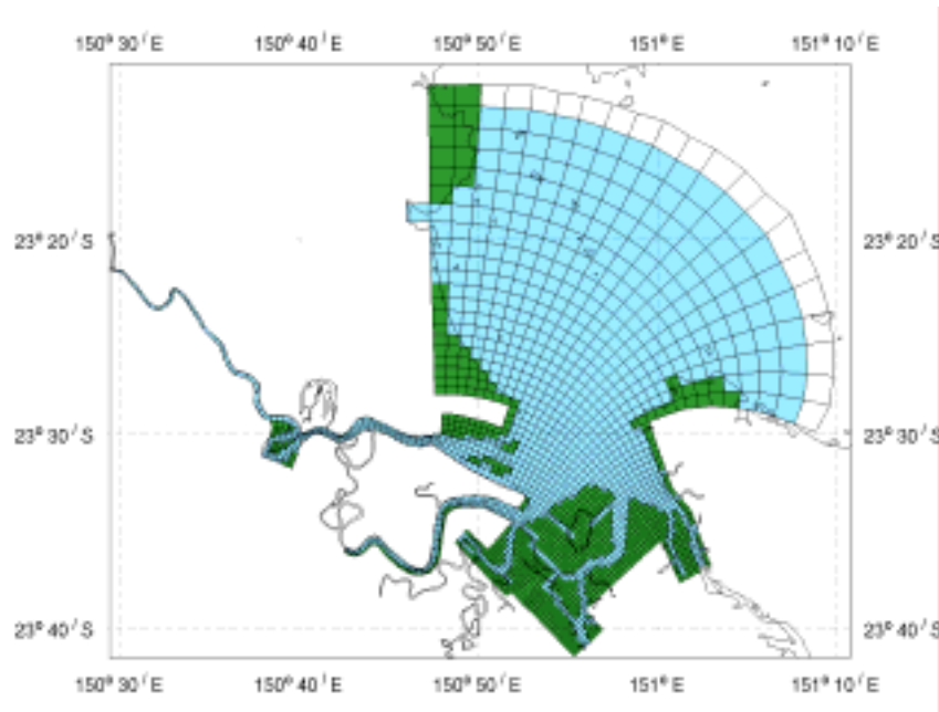
Figure 3. Plan view of the 3-D numerical grid
