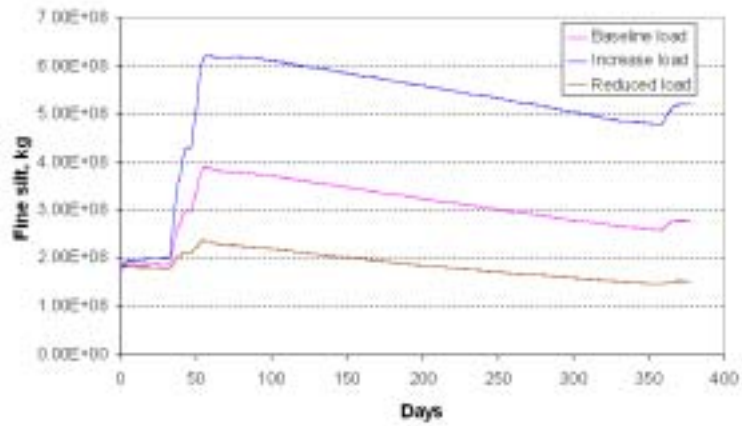
Figure 20. Mass balance of fine silt under scenarios with baseline flow and different land-use practices
