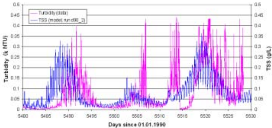
Figure 12. Modelled TSS and turbidity versus measurements, January–February 2005 (TSS = 1.13xturbidity)
