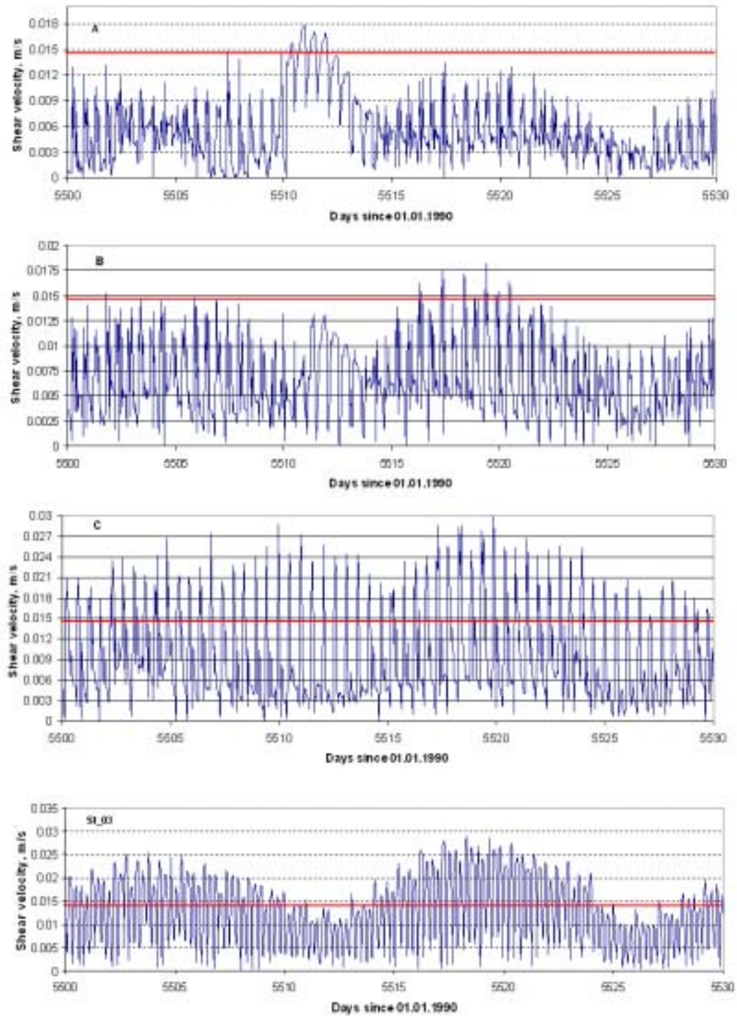
Figure 15a. Time series of shear velocities in the Fitzroy Estuary and Keppel Bay, sites A, B, C and 3
