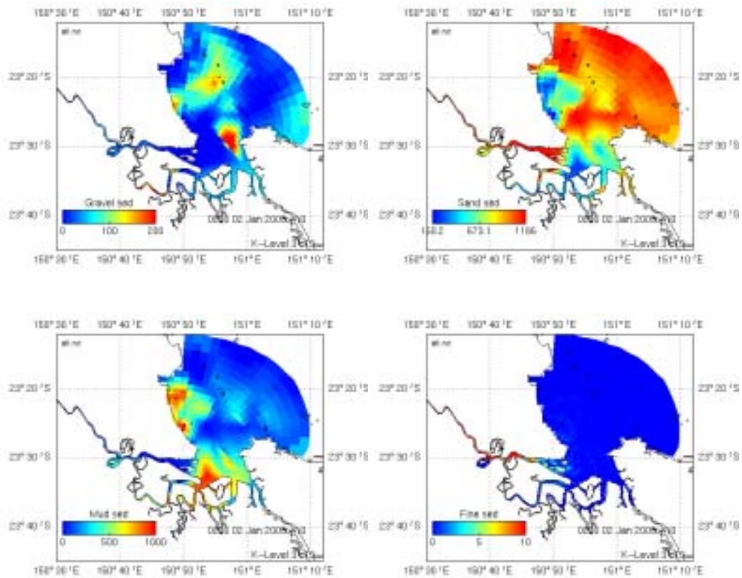
Figure 4. Initial distribution of gravel, sand, mud and clay fractions of sediment, as used in the model
