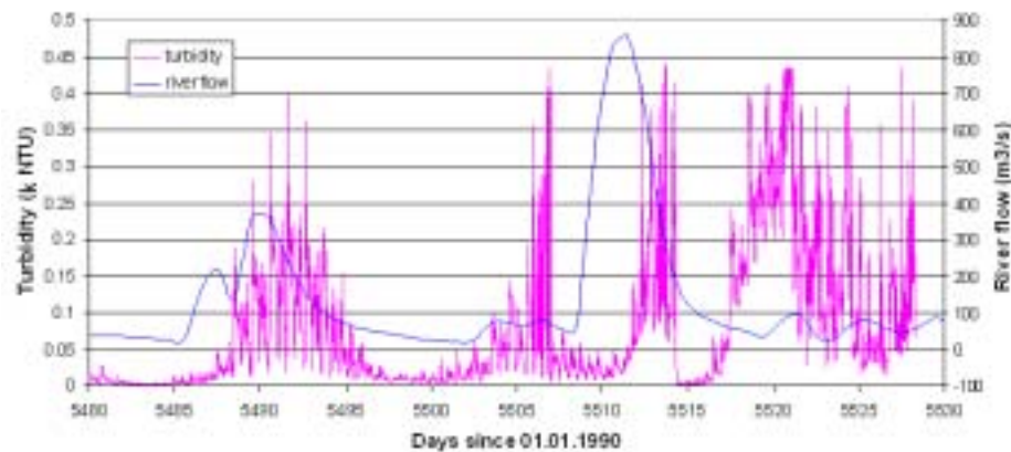
Figure 11. Measured turbidity versus river flow
