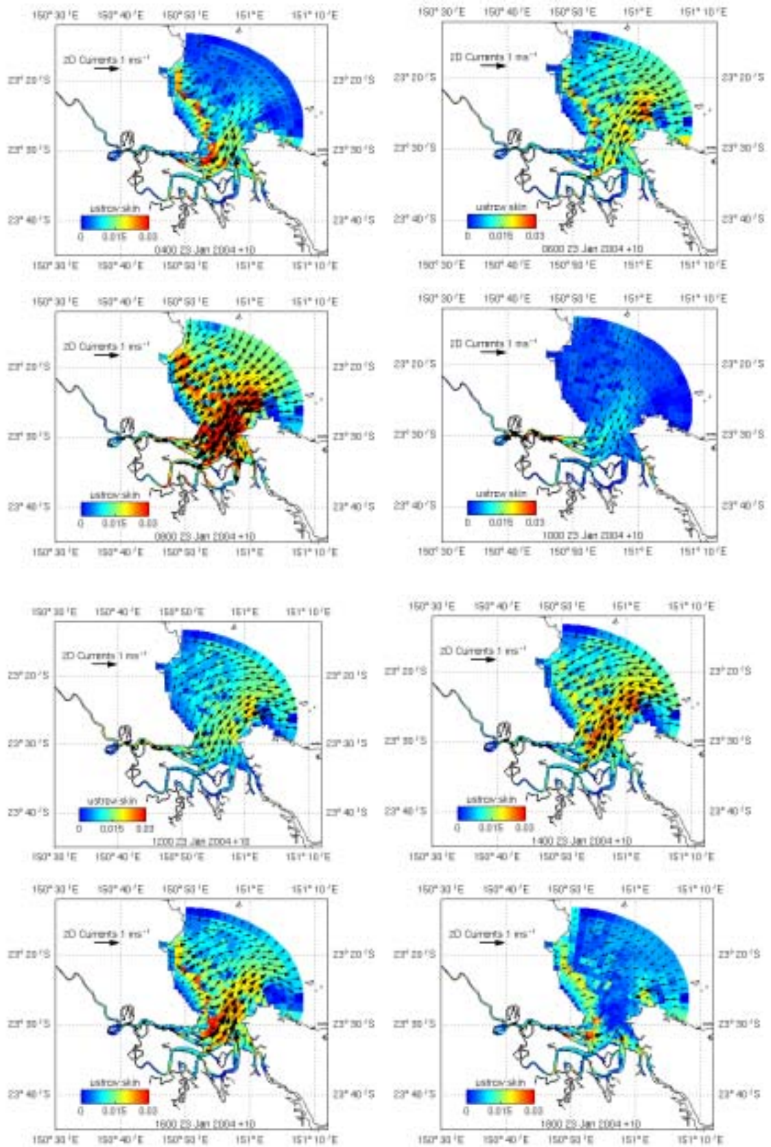
Figure 14. Simulated bottom shear velocities in the Fitzroy Estuary and Keppel Bay over one tidal cycle (spring tide)
