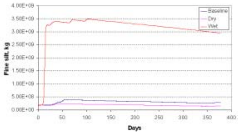
Figure 21. Mass balance of fine silt under scenarios with different flow regimes
