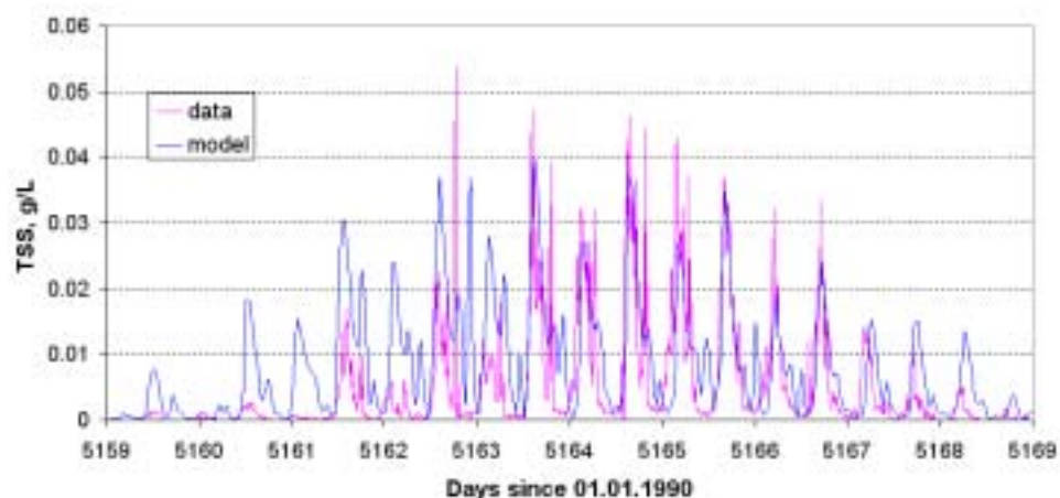
Figure 8. Modelled TSS versus data, February 2004
