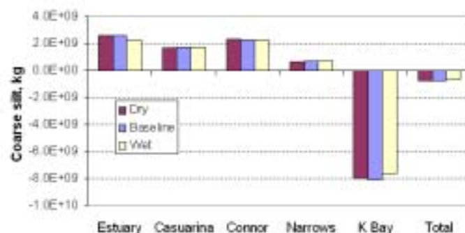
Figure 23. Mass balance of coarse silt after one-year modelling, under scenarios with different flow regimes
