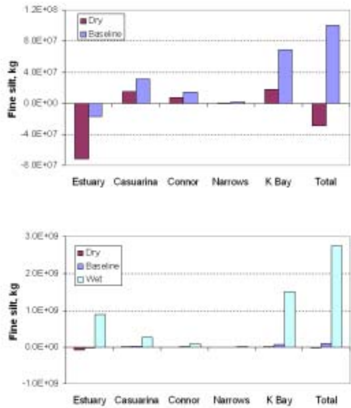
Figure 18. Mass balance of fine silt after one-year modelling (scenarios with different flow regimes)
