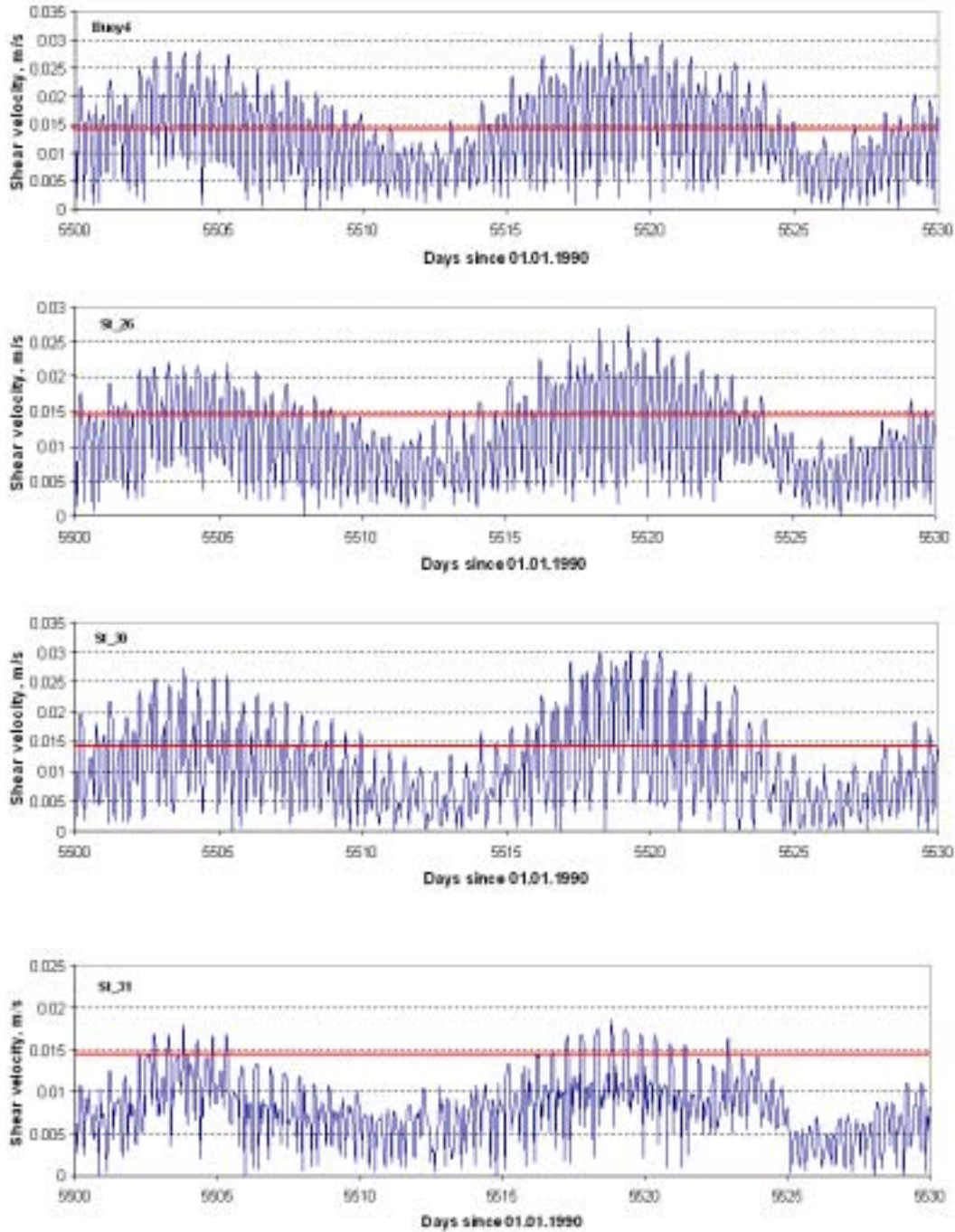
Figure 15b. Time series of shear velocities in the Fitzroy Estuary and Keppel Bay, sites 4, 26, 30 and 31
