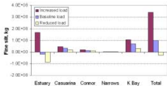
Figure 19. Mass balance of fine silt after one-year modelling (scenarios with different land-use practices)
