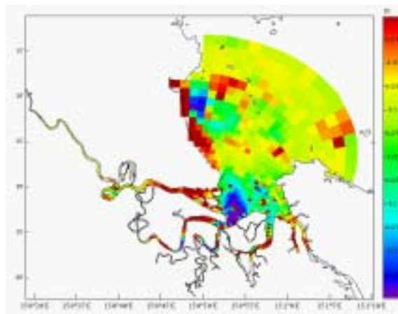
Figure 24. Simulated sediment thickness after one-year modelling (scenario with baseline flow)
