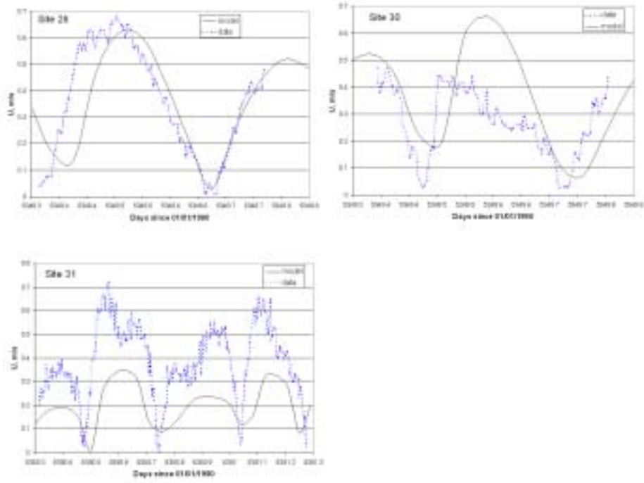
Figure 7. Modelled velocity versus measurements, August 2004
