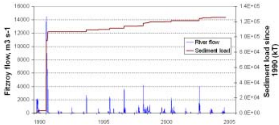
Figure 25. Sediment loads through the Fitzroy barrage, integrated with time
