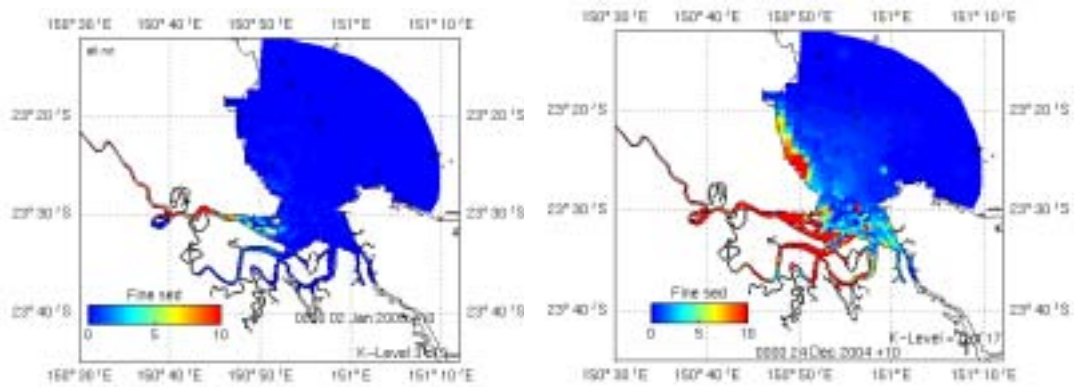
Figure 22. Simulated redistribution of fine sediments after baseline year
